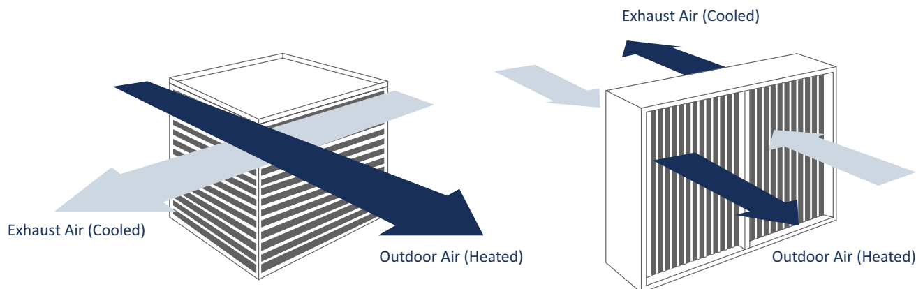
FIGURE 10: HEAT EXCHANGE
