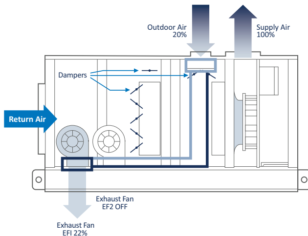
FIGURE 15: NORMAL MODE WITH GLYCOL HEAT RECOVERY
