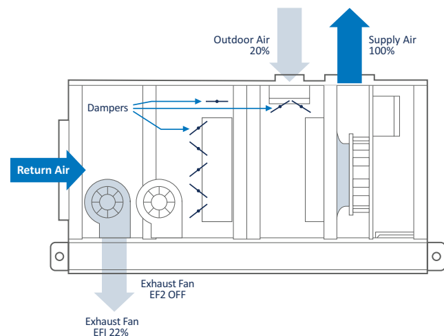
FIGURE 14: NORMAL MODE
