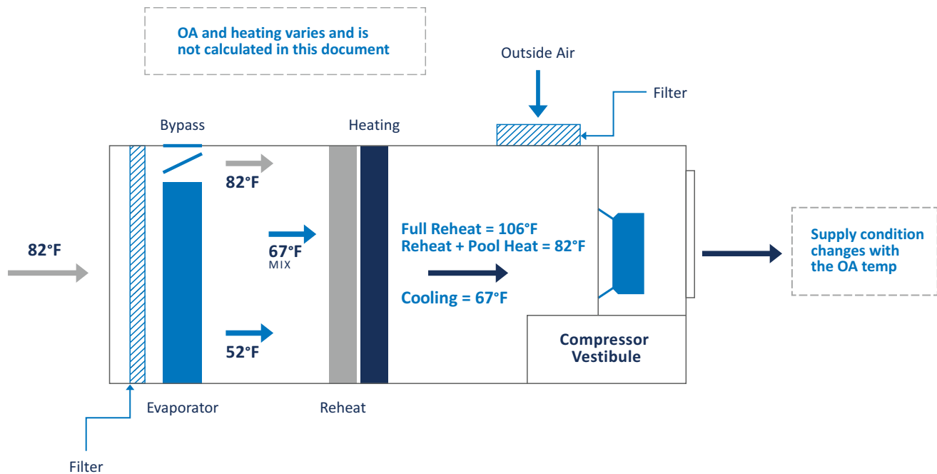
FIGURE 20: REFRIGERATION-BASED DEHUMIDIFIERS
