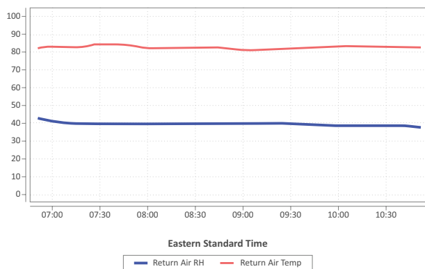
FIGURE 19: POOLPAK'S MODULATING REHEAT SYSTEM PROVIDES STABLE TEMPERATURES AND RH LEVELS
