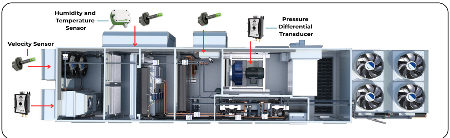
Figure 1. Sensor placement diagram showing the location of all sensors on the PPK model.
